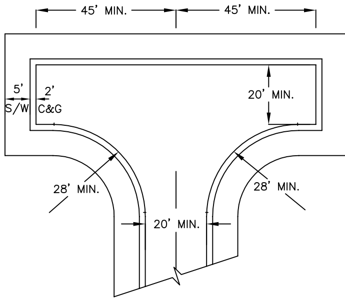
HAMMERHEAD
