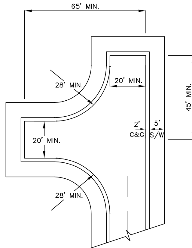
MODIFIED HAMMERHEAD
