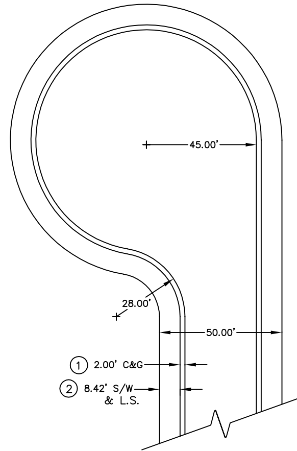
MODIFIED CUL-DE-SAC
