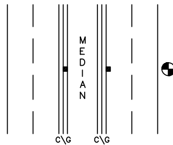
Figure 6 MULTI-LANE STREET WITH MEDIAN
