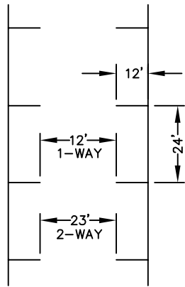
PARALLEL PARKING
