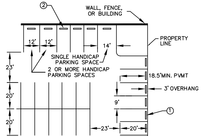
90° PARKING
