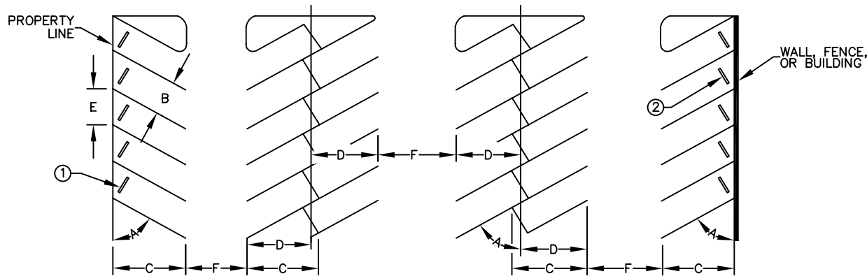
ANGLE PARKING
