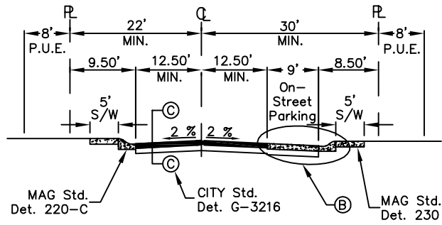
PRIVATE STREET WITH ON-STREET PARKING
